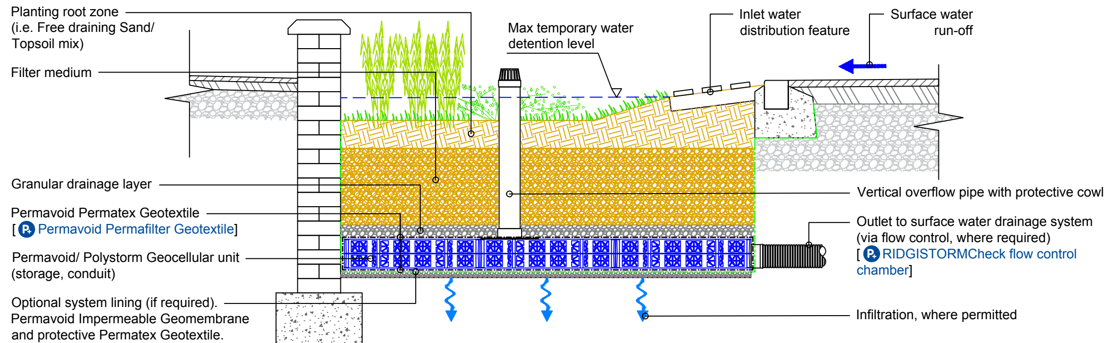
TYPICAL SECTION
