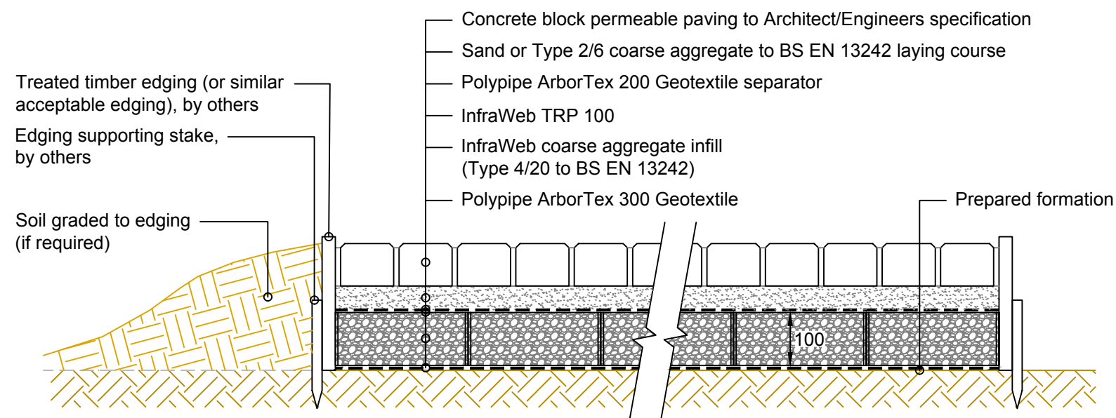
TYPICAL SECTION Scale 1:10
