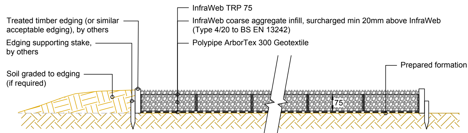
TYPICAL SECTION Scale 1:10
