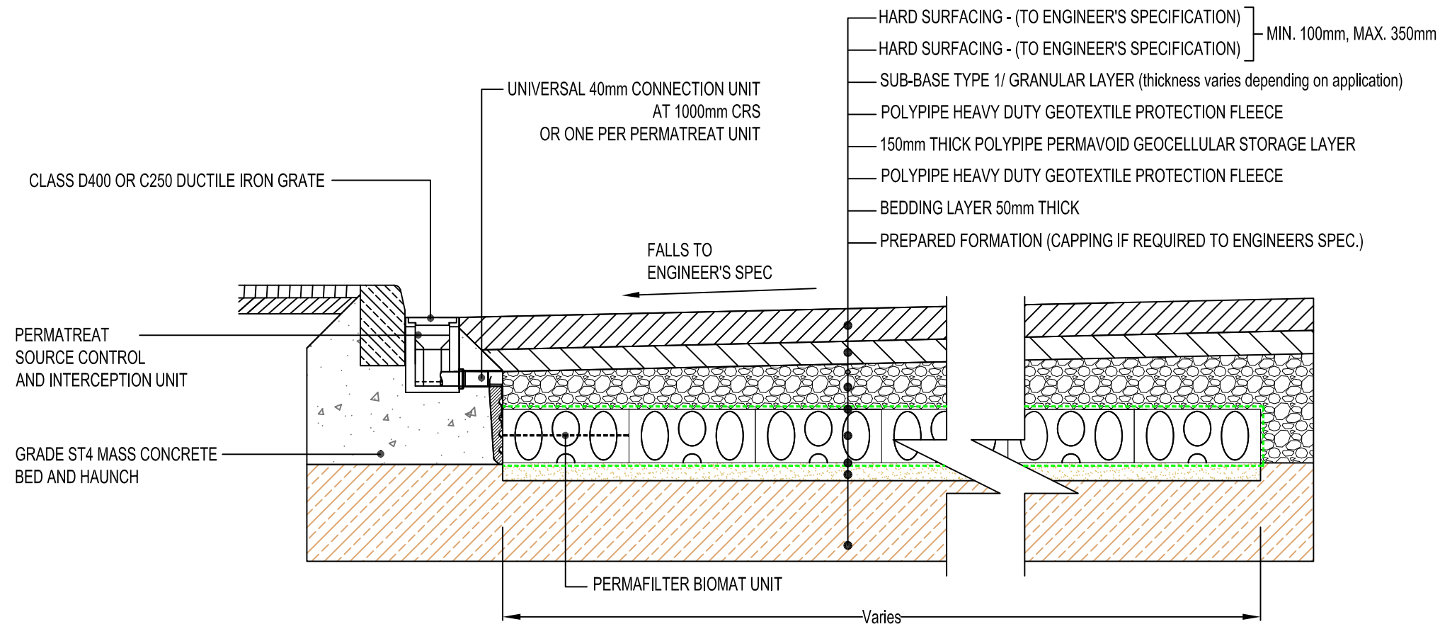
TYPICAL SECTION THROUGH POLYPIPE PERMATREAT AND PERMAVOID INFILTRATION TANK Scale (1:15)
