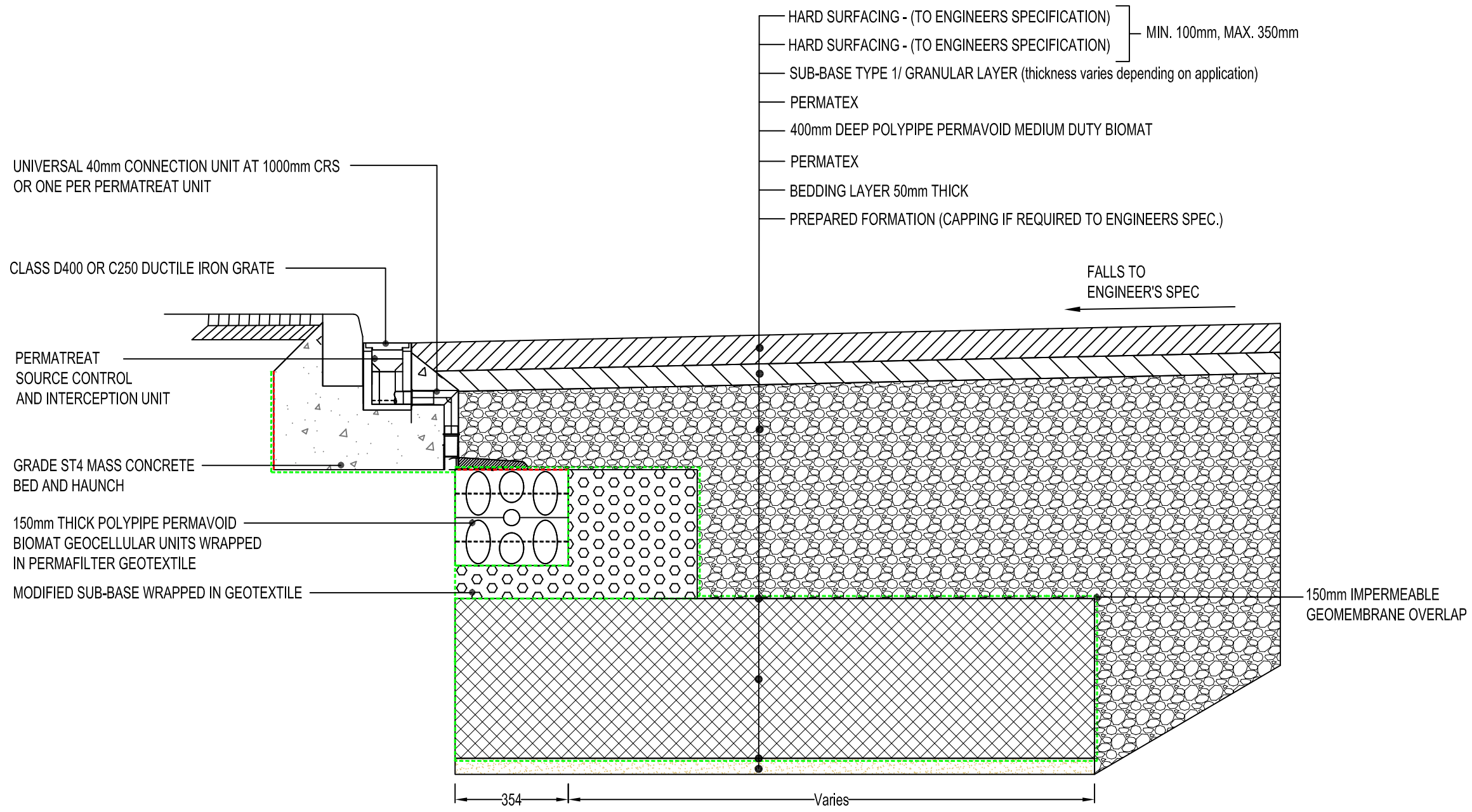
TYPICAL SECTION THROUGH POLYPIPE PERMATREAT AND HEAVY DUTY PERMAVOID CONDUIT WITH A POLYPIPE POLYSTORM INFILTRATION TANK
